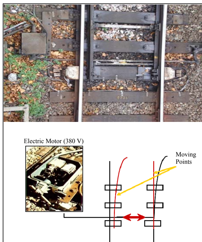
Figure 1: Switch mechanism driven by an electrical motor.
